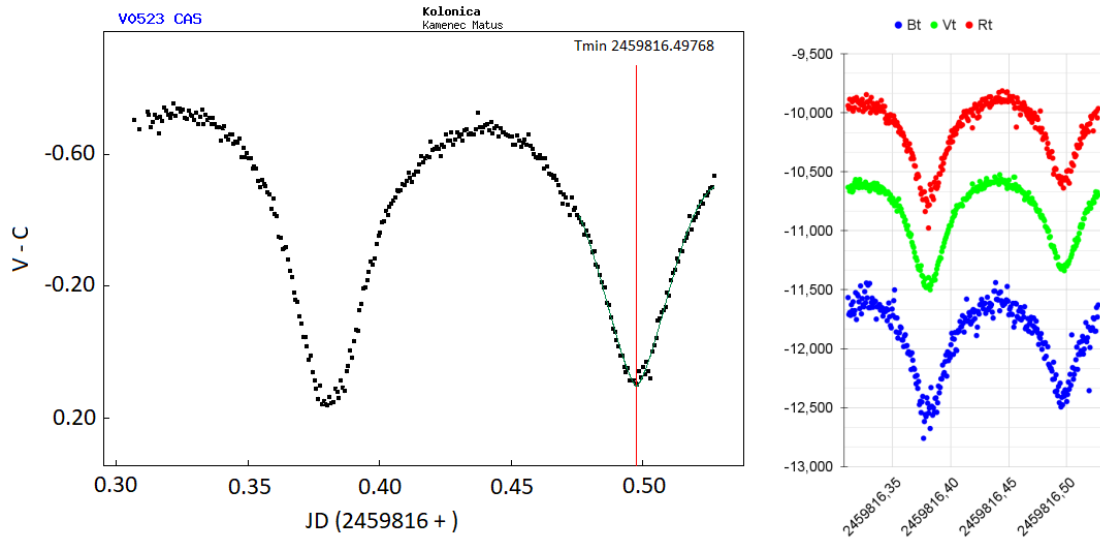
Figure 8: On the left, the light curve in the clear filter; on the right, the transformation into B, V, and R c filters (V0523 Cas, 24 August 2022, Kolonica)
