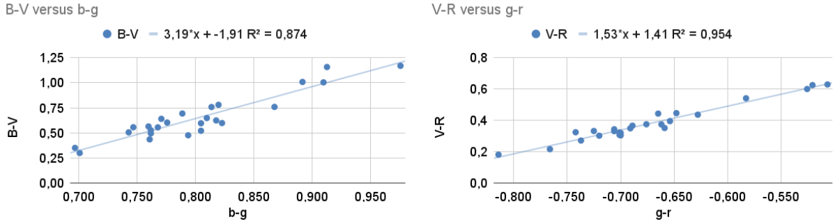
Figure 5: Catalogue vs instrumental colour indices.
