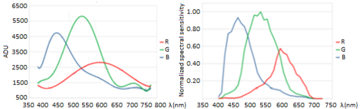
Figure 3: Spectral response of Canon 500D, our measurement on the left, Jiang et al. (2013) on the right
