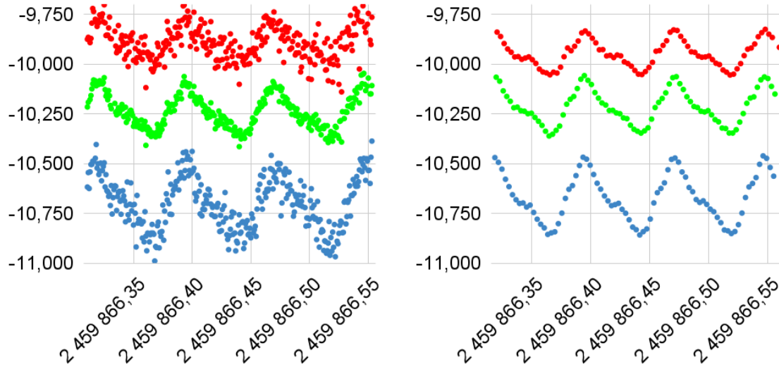
Figure 11: Simultaneous observation of V0799 Aur at the same time, in the same place (13 October.2022, Canon 500D on the left, G2-1600 on the right)
