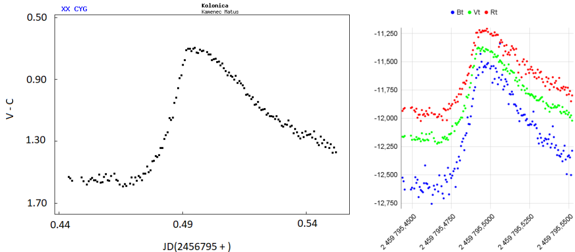
Figure 9: On the left, the light curve in the “clear” filter; on the right, the transformation into B, V, and R c filters (XX Cyg, 3 August.2022, Kolonické sedlo)
