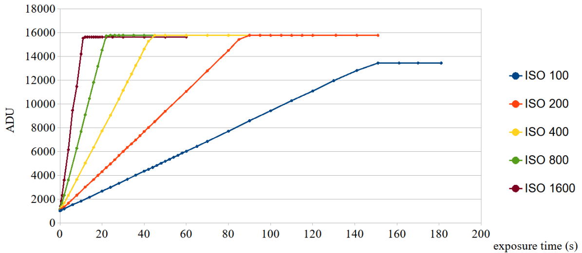
Figure 2: Canon 500D linearity at different ISO levels.
