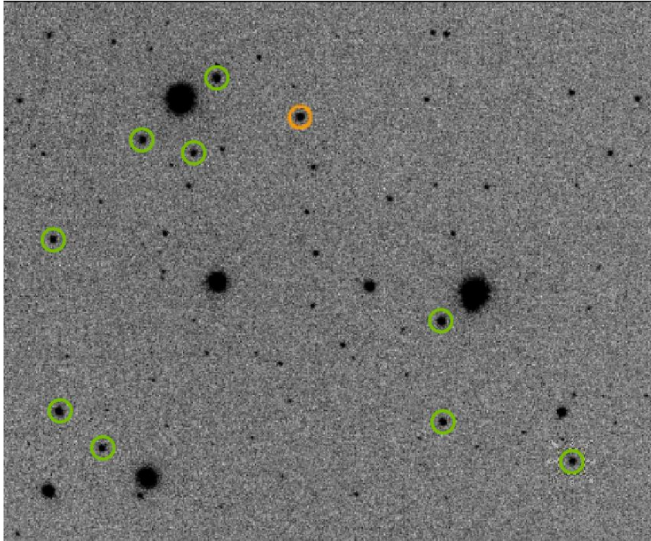
Figure 4: Melotte 111 frame cutout with selected calibration stars
