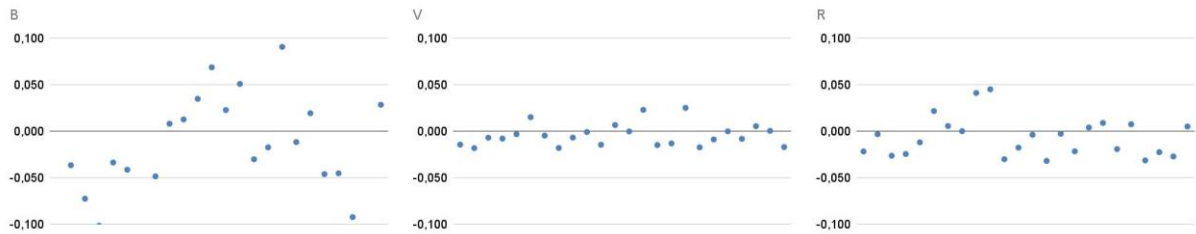
Figure 7: Deviations of transformed B, V, and R c magnitudes from catalogue values
