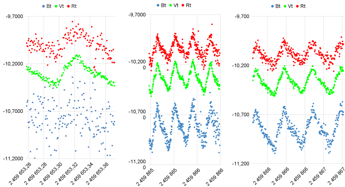
Figure 10: Transformed lightcurves of V0799 Aur, on the left 14 March 2022, Prešov, 102/500, in the middle and on the right 12 October 2022, resp. 13 October 2022, 200/1200, Kolonica Saddle Canon 500D
