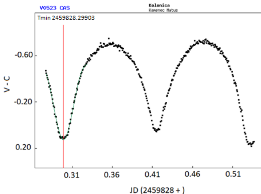
Figure 1: Example of the light curve of V0523 Cas in the “clear” filter, with the primary minimum marked (5 September 2022, Newton 200/1200, Canon 500D)
